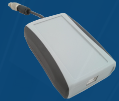
TCL Interface
